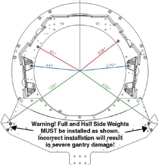
GANTRY FRONT VIEW TUBE AT 0°
